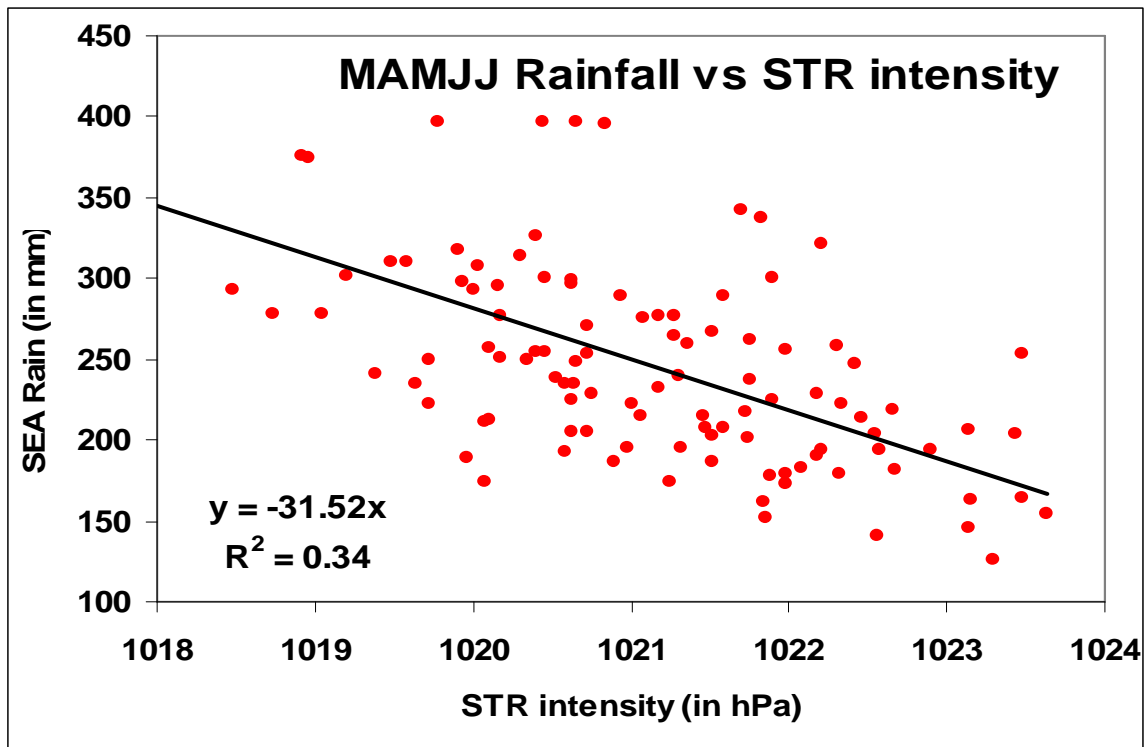
Figure 3: Relationship between SEA March-April-May-June-July rainfall and the sub-tropical ridge (STR) intensity during the same five months. The slope of the linear relationship and the amount of explained variance ( r^2 ) is shown in the lower left corner.
